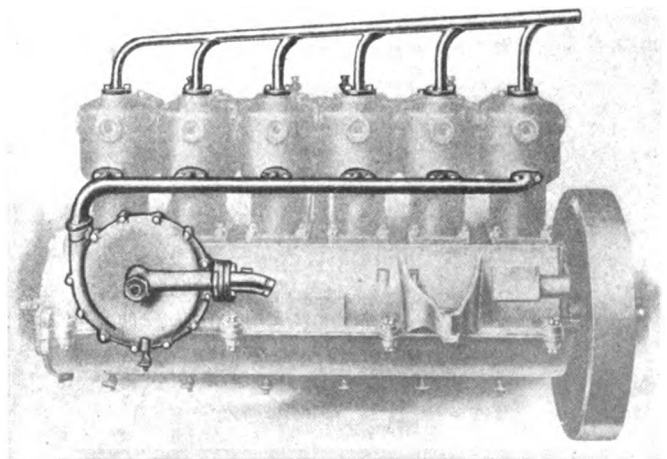
Fig. 7.—Centrifugal type applied to a "six."
